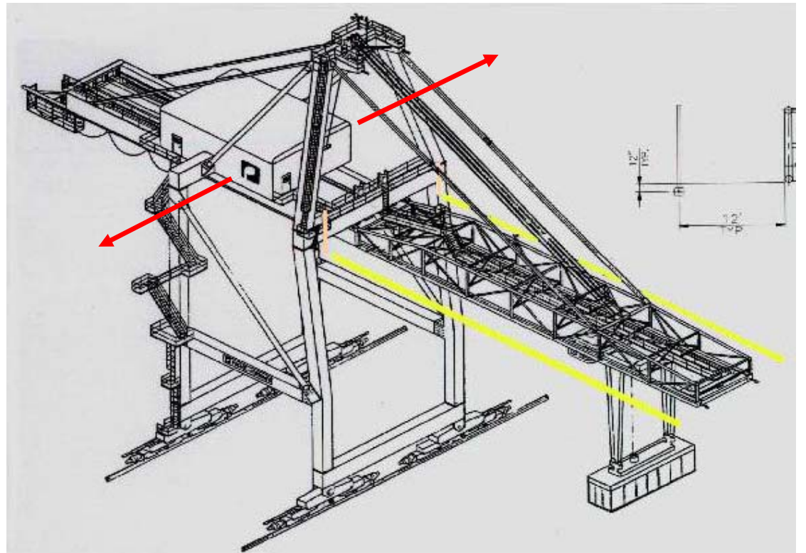
PACECO® CORP. Boom Anticollision Laser Trajectory Protection Area (Arrows in Red)
